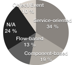
Figure 15: Programming model.
