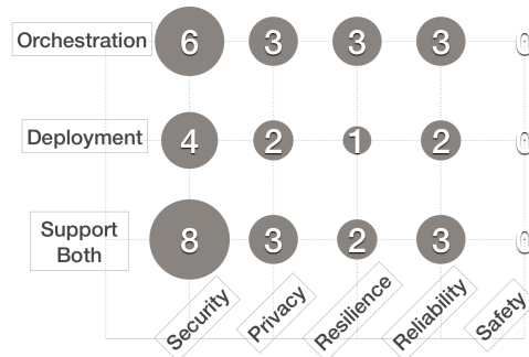
Figure 18: Trustworthiness aspects.
