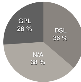
Figure 16: Language types.
