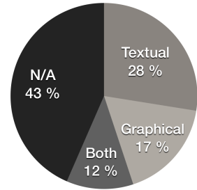
Figure 17: Representation types.
